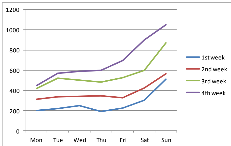
Figure 2. One month daily customer counts
