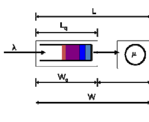
Figure 1. Illustrates the M/M/1 queuing model
