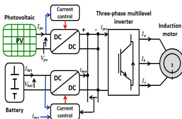
Figure 1: Induction motor driven by PV-batteries standalone system using a controlled multilevel inverter
