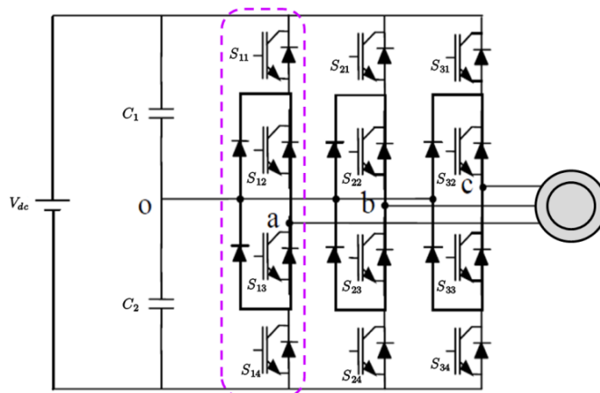
Figure 2: Three-level three phase inverter
